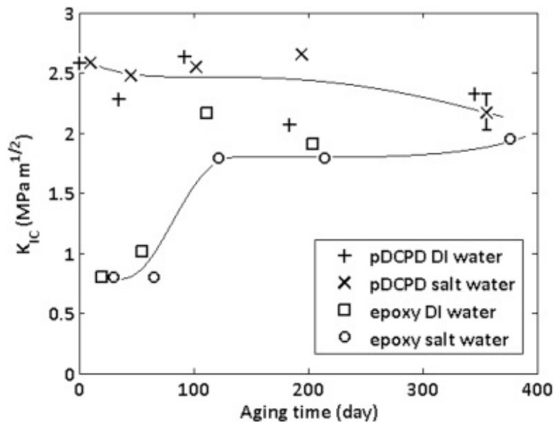
Fig. 4. Fracture toughness of neat cured resin.
