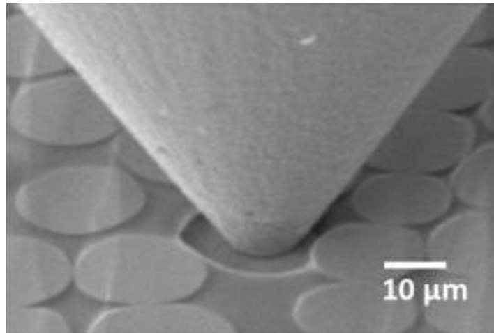
Fig. 1. Fiber push-out of glass/pDCPD composite.
