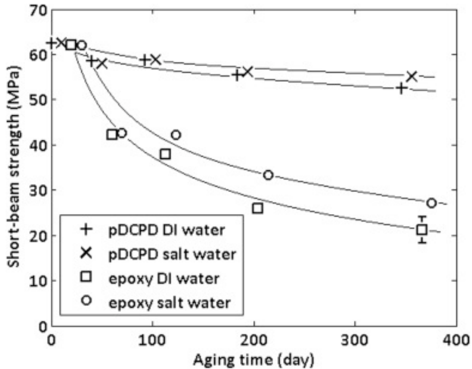
Fig. 7. Short-beam strength evolution during aging.
