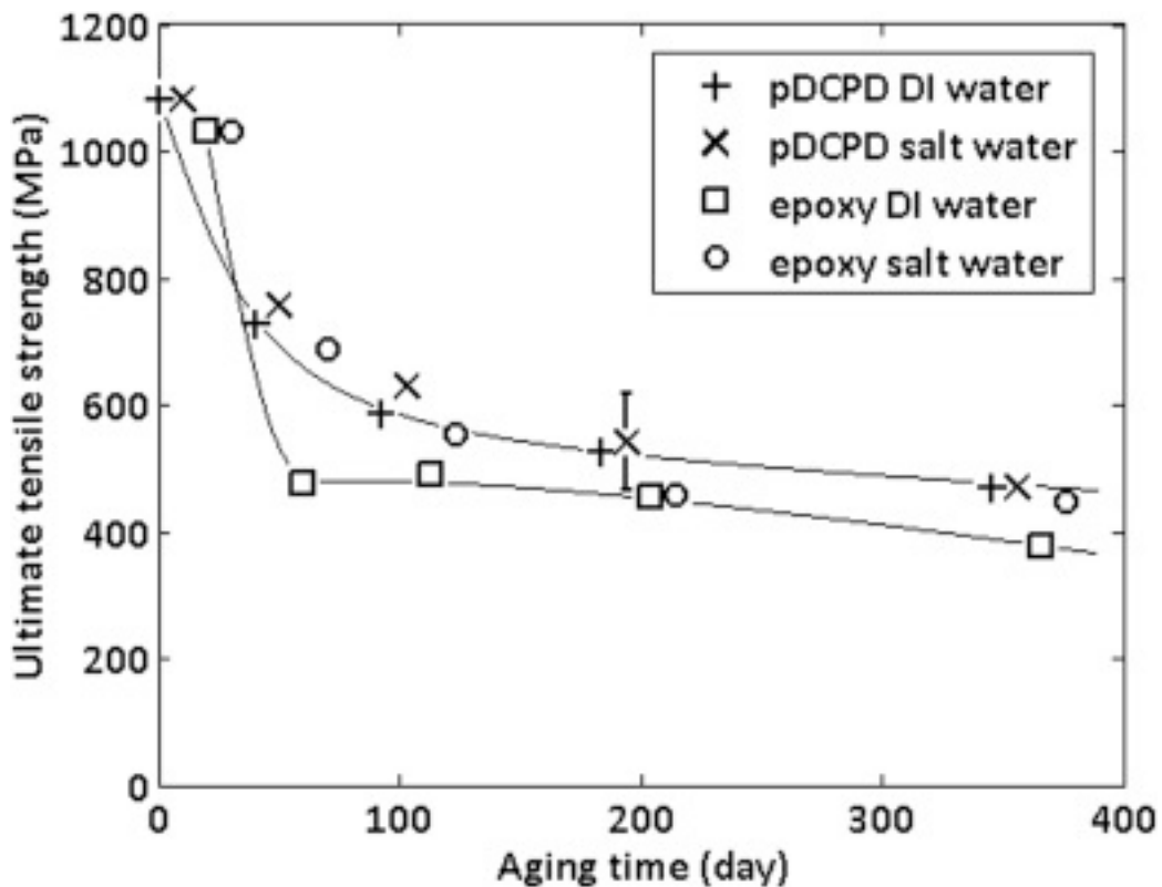
Fig. 5. Tensile strength evolution of 0° composite during aging.
