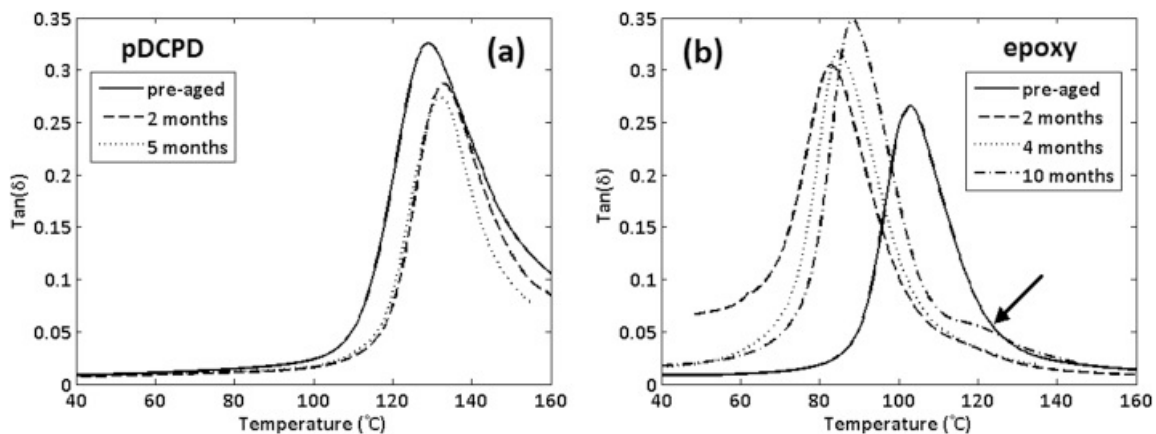
Fig. 3. \tan(\delta) curve evolution during aging from DMA.
