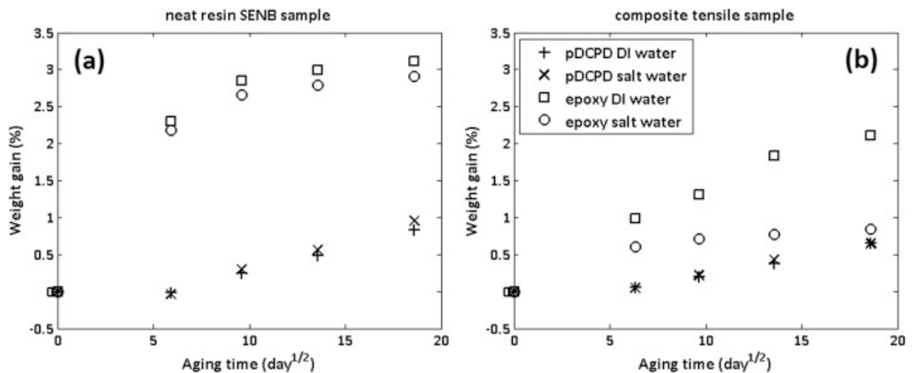
Fig. 2. Weight change during aging.
