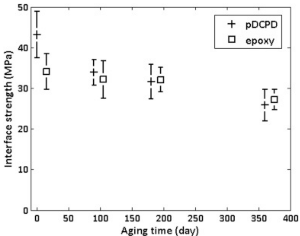
Fig. 6. Interface strength evolution from fiber push-out test (60 °C DI water).
