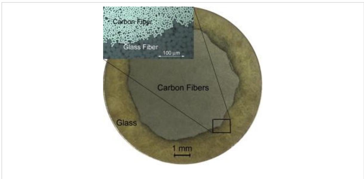
Fig. 1. Cross-section of unidirectional CF/GF hybrid composite rod, showing the CF core region, surrounded by the GF shell [7]. (For interpretation of the references to colour in this figure legend, the reader is referred to the web version of this article.)
