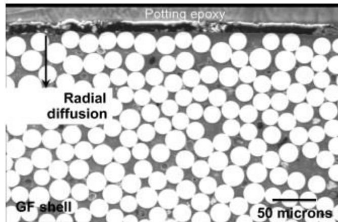
Fig. 5. SEM micrograph of a specimen exposed to 60 °C and 85% relative humidity after nearly 5 months.
